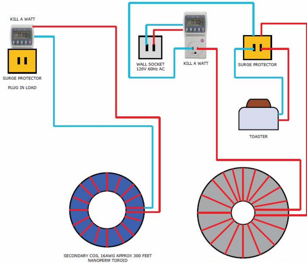
PRIMARY COIL 16AWG APPROX 400 FEET COLD ROLLED STEEL TOROID
